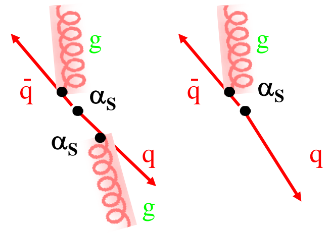
“parton level” pictures
