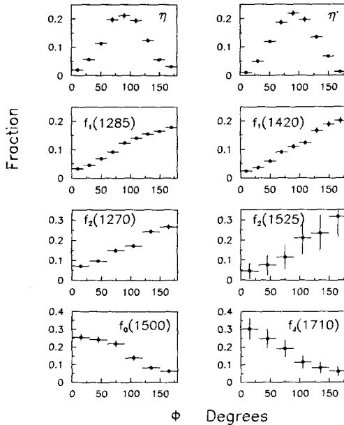
Figure 2. The azimuthal angle between the fast and slow protons \phi for various resonances.
