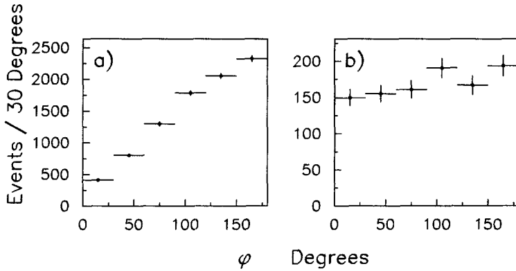
Figure 3. The azimuthal angle between the fast and slow protons \phi for the f_1(1285) for a) |t_1 - t_2| \leq 0.2 and b) |t_1 - t_2| \geq 0.4
