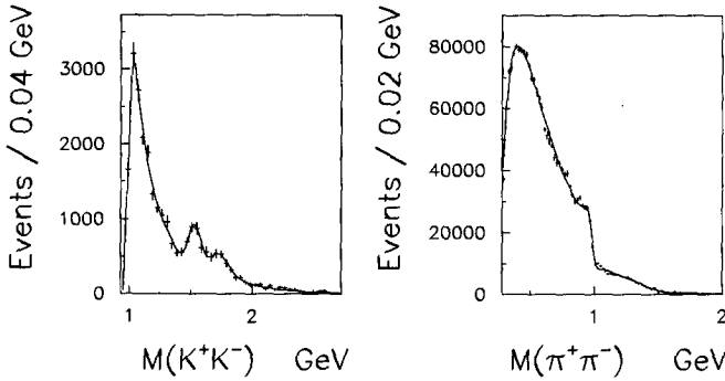
Figure 1. The S_0^- -Waves resulting from a partial wave analysis of the K^+K^- and \pi^+\pi^- - systems.
