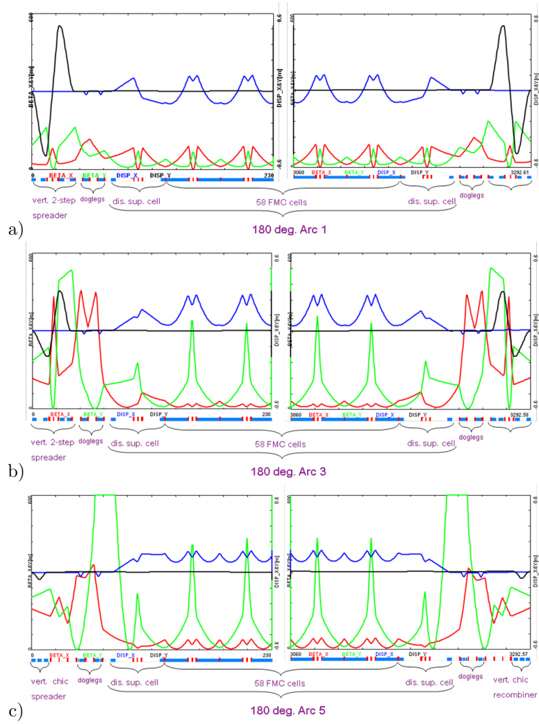
Figure 7.34: Compete Arc 1, 3 and 5 lattices including: spreaders, recombiners and path-length correcting “doglegs” matched to the corresponding linacs.
