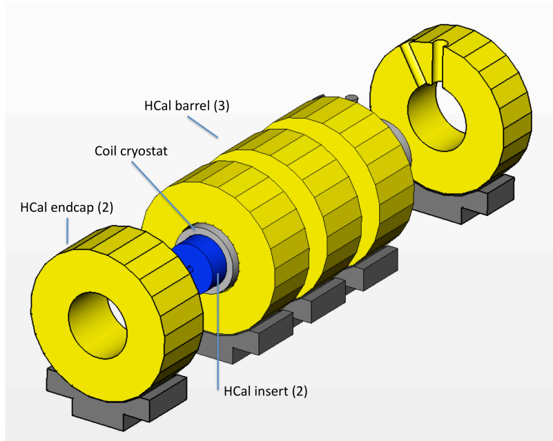
Figure 14.2: The main detector elements to be assembled on surface.
