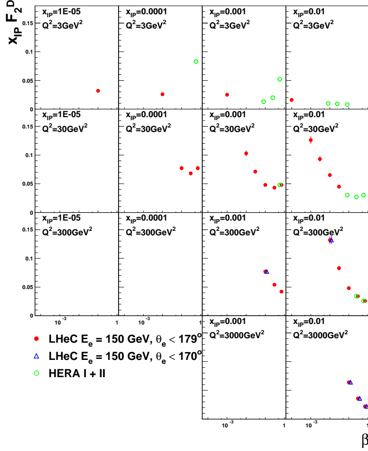
Figure 4.39: Simulation of a possible LHeC measurement of the diffractive structure function, F_2^D using a 2\text{ fb}^{-1} sample, compared with an estimate of the optimum results achievable at HERA using the full luminosity for a single experiment ( 500\text{ pb}^{-1} ). The loss of kinematic region if the LHeC scattered electron acceptance extends to within 10^\circ of the beam-pipe, rather than 1^\circ is also illustrated.
