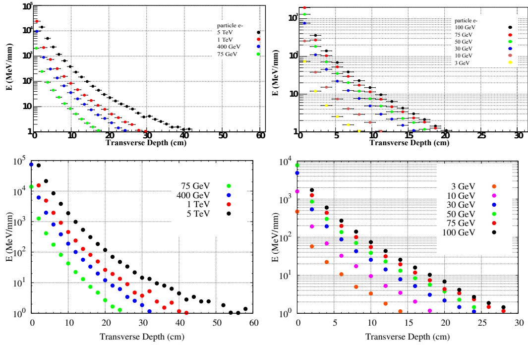
Figure 12.46: Comparison of transverse shower profiles for electrons with energies 75 GeV-5 TeV on \text{FEC}_{(W-Si)} (left) and 3 GeV-100 GeV on \text{BEC}_{(Pb-Si)} (right) ( GEANT4 (top) and FLUKA (bottom)).
