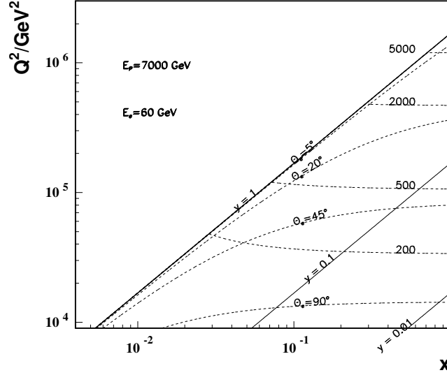
Figure 11.5: Kinematics of electron detection in the forward detector region corresponding to large Q^2 \geq 10^4 \text{ GeV}^2 . The energy values are given in GeV. At very high Q^2 the iso- E'_e lines are rather independent of x , i.e. Q^2(x, E'_e) \simeq 4E_e E'_e .
