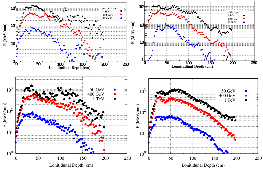
Figure 12.48: Average energy deposition as a function of depth for pions in the energy range 50\text{ GeV} - 1\text{ TeV} in the \text{FEC}_{(W-Si)} \& \text{FHC}_{(W-Si)} system (left) and in the \text{FEC}_{(W-Si)} \& \text{FHC}_{(Cu-Si)} composite stack system (right) ( GEANT4 (top) and FLUKA (bottom)).
