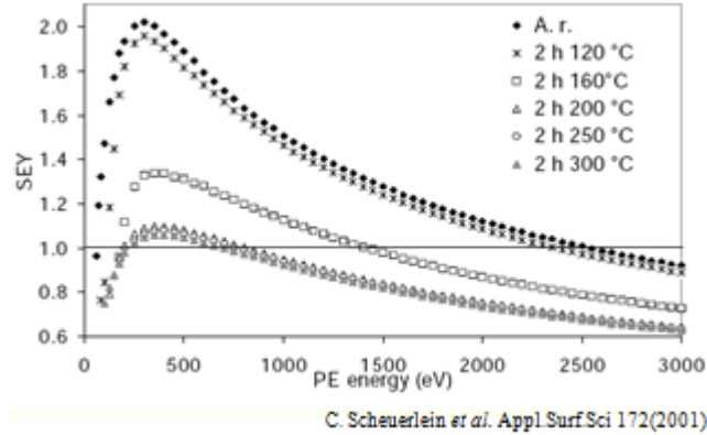
Figure 8.29: Reduction of the secondary electron yield (SEY, \delta ) by Photons a) and Electron b) desorption yields.
