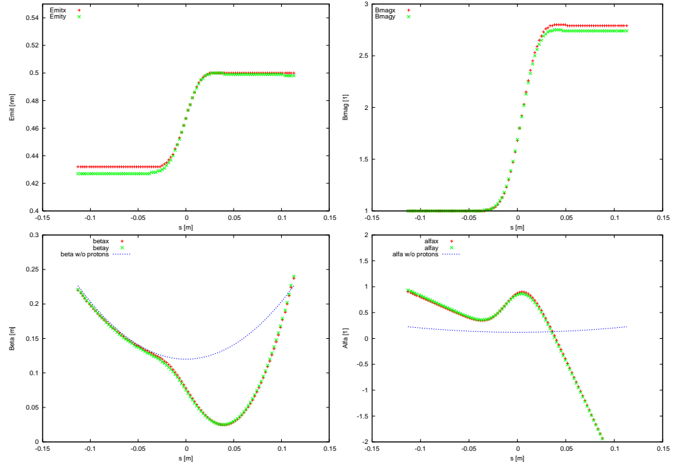
Figure 7.6: Simulated evolution of the electron beam emittance (top left), mismatch factor B_{\text{mag}} (top right) beta function (bottom left) and alpha function (bottom right) during the collision with a proton bunch, as a function of distance from the IP.
