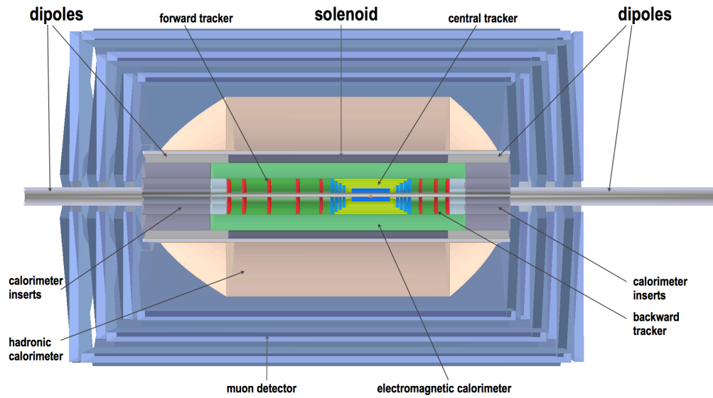
Figure 12.12: Configuration of the solenoid and electron beam bending dipoles in the baseline Linac-Ring detector. Longitudinal r-z section showing the position of the solenoid and the two dipoles, each split in two sections, a superconducting inner section incorporated with the solenoid in one cryostat and a normal conducting iron based outer section magnet with smaller bore.
