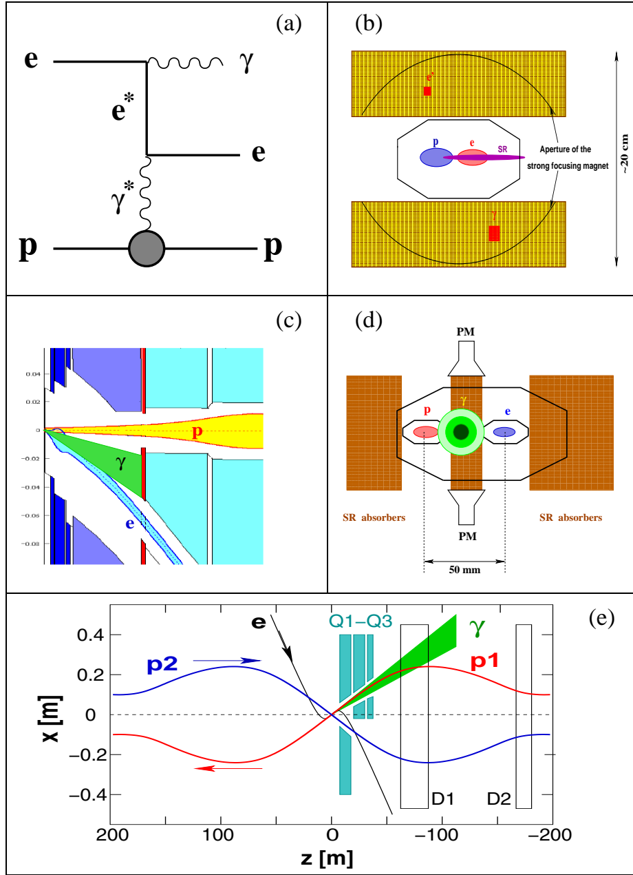
Figure 13.1: Options for the luminosity monitoring at the LHeC. (a) Feynman diagram for QEDC ( \gamma^* pole) or BH ( \gamma^*, e^* poles) processes; (b) QEDC tagger at z = -6\text{m} ; (c,d) active SR absorber at z = -22\text{m} for RR-option (circles show 1-, 2- and 3- \sigma contours for BH photons); (e) schematic view for the LR-option with 3- \sigma fan of BH photons.
