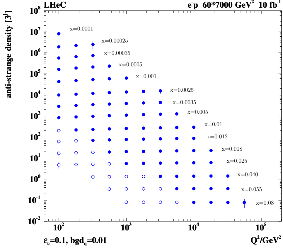
Figure 3.13: Simulated measurement of the anti-strange quark density in CC e^-p scattering with charm tagging at the LHeC, for a luminosity of 10 fb -1 . Closed (open) points: tagging acceptance down to 10 (1°). The charm quark tagging efficiency is assumed to be \epsilon_c = 10\% and the efficiency to keep light quark background \text{bgd}_q = 1\% .
