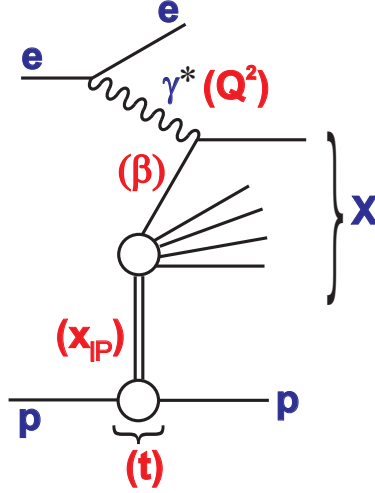
Figure 4.37: Illustration of the kinematic variables used to describe the inclusive diffractive DIS process ep \rightarrow eXp .
