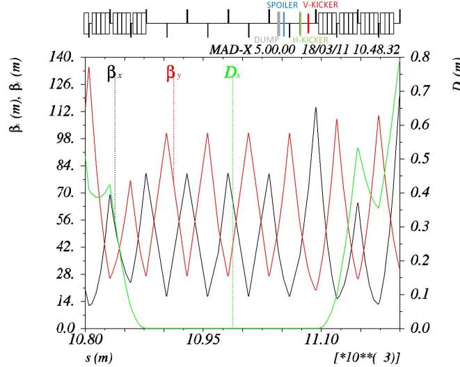
Figure 8.43: The optics in the region of the CMS bypass where the beam dump system could be installed is shown. The system consists of two kickers, one spoiler and a Carbon-composite absorber which are installed in the dispersion free region of the bypass at the right side of CMS (beam proceeds from right to left in the Figure).
