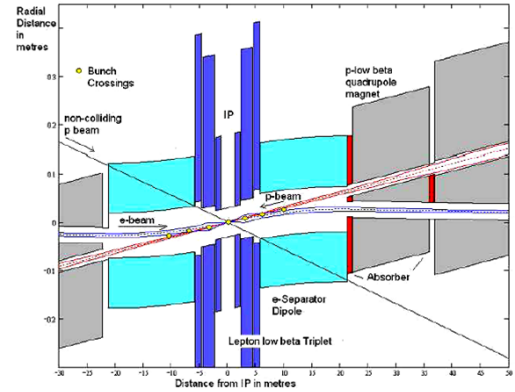
Figure 1: The high luminosity IR layout [5].
