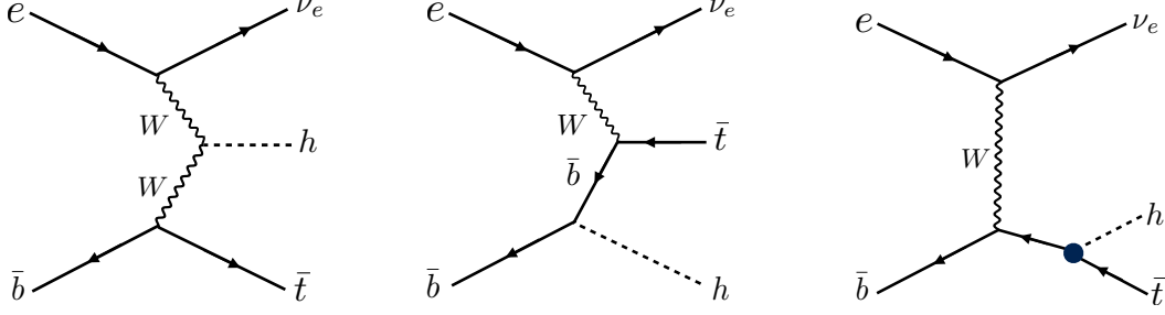
Figure 7.14: Leading order Feynman diagrams contributing to the process p e^- \rightarrow \bar{t} h \nu_e in high energy e^- p collisions. The black dot in the Feynman diagram on the right denotes the top-quark-Higgs coupling of interest in this section.
