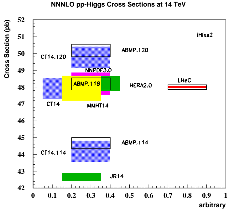
Figure 9.5: Cross sections of Higgs production calculated to N^3\text{LO} using the iHix program [723] for existing PDF parameterisation sets (left side) and for the LHeC PDFs (right side). The widths of the areas correspond to the uncertainties as quoted by the various sets, having rescaled the CT14 uncertainties from 90 to 68 % C.L. Results (left) are included also for different values of the strong coupling constant \alpha_s(M_Z^2) , from 0.114 to 0.120. The inner LHeC uncertainty band (red) includes the expected systematic uncertainty due to the PDFs while the outer box illustrates the expected uncertainty resulting from the determination of \alpha_s with the LHeC.
