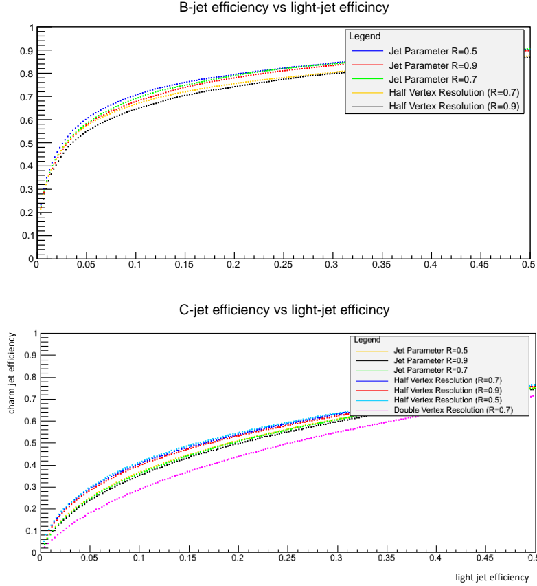
Figure 7.7: Expected average efficiency to tag a b -jet (upper plot) and charm-jet (lower plot) versus the light-jet efficiency (x-axis) based on Tevatron-style jet tagging [598]. Events are selected at DELPHES detector level using a CC multi-jet sample and for an integrated luminosity of 100 \text{ fb}^{-1} . The coloured lines correspond to the choice of the anti-kt distance parameter R and different assumptions in the impact parameter resolution of 10 (5) \mu\text{m} (nominal, no text added in legend), 5 (2.5) \mu\text{m} (Half Vertex Resolution), 20 (10) \mu\text{m} (Double Vertex Resolution) for tracks with 0.5 < p_T < 5 ( > 5 ) GeV within |\eta| < 3.5 .
