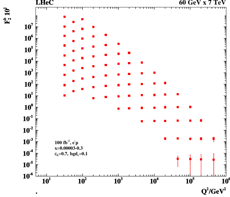
Figure 3.7: Simulation of the measurement of the bottom quark distribution expressed as F_2^b = e_b^2 x(b + \bar{b}) in neutral current e^-p scattering. The data are plotted with full systematic and statistical errors added in quadrature, mostly invisible. The minimum x (left top bin) is at 3 \cdot 10^{-5} , and the data extend to x = 0.3 (right bottom bin). The simulation uses a massless scheme and is only indicative near threshold albeit the uncertainties entering the QCD PDF analysis are estimated consistently.
