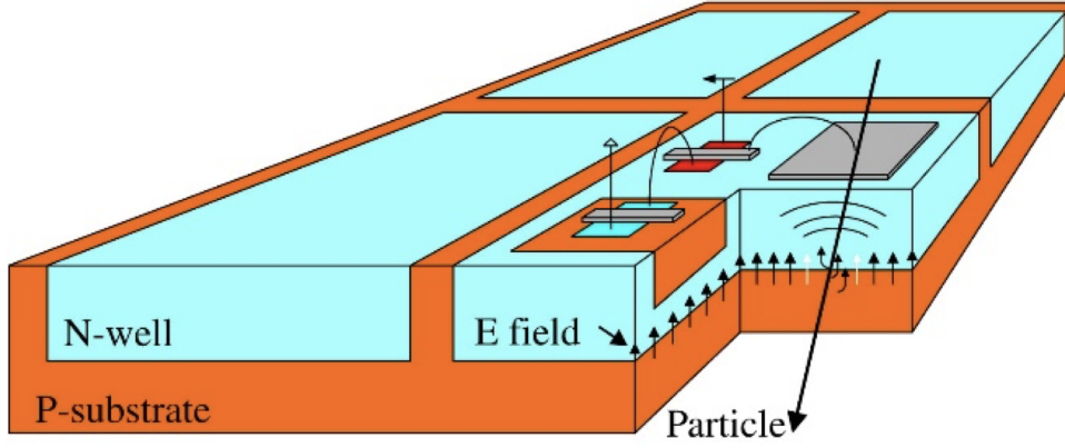
Figure 12.10: Typical sensor cross-section of a DMAPS detector in a HV-CMOS process [894].
