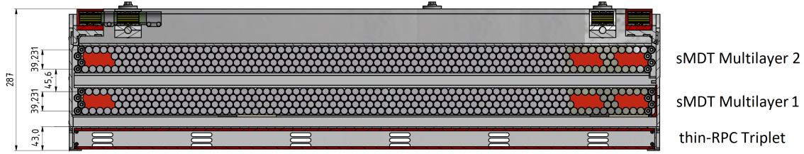
Figure 12.15: A transverse view of a RPC-MDT assembly as adapted from a drawing of the ATLAS Phase-1 muon upgrade [902]. In this case a station is composed of an RPC triplet for trigger and two-coordinate readout and two MDT superlayers for precise track measurements.
