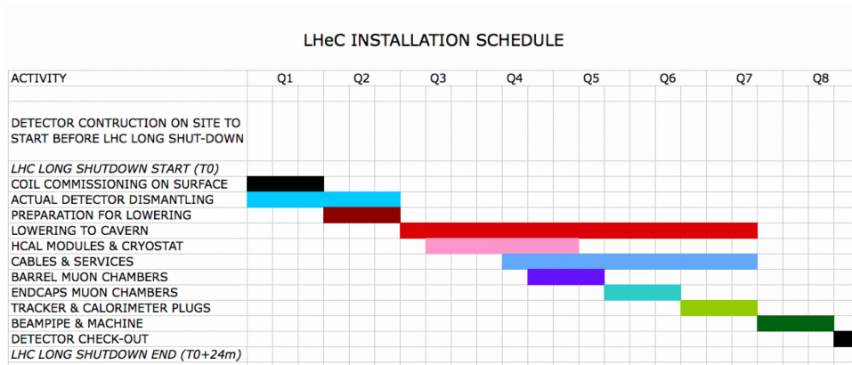
Figure 12.20: Time schedule of the sequential installation of the LHeC detector at point 2, as described in the text.
