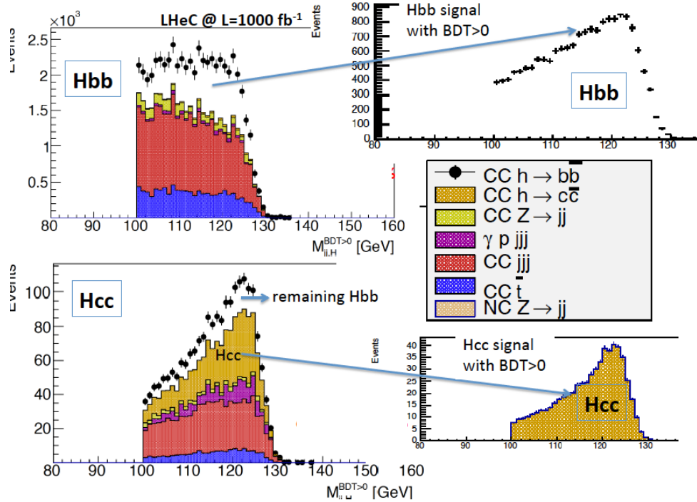
Figure 7.9: Result of the joint H \rightarrow b\bar{b} and H \rightarrow c\bar{c} analysis for an integrated luminosity of 1 \text{ ab}^{-1} and -80 % electron polarisation at the LHeC. Left: Invariant mass distributions for the two channels with signal and background, see text. Right: Expected Higgs signal distributions after background subtraction. The background is assumed to be at the 2 % level via control region measurements.
