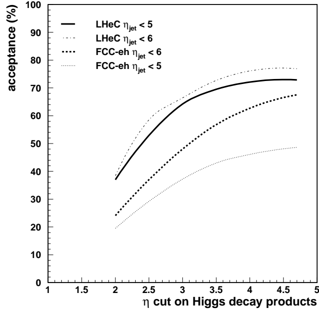
Figure 7.4: Acceptance of DIS Higgs candidates ( y axis) in dependence on the pseudorapidity ( \eta ) cut requirement on the Higgs decay products ( x axis) for two scenarios of the coverage of the hadronic final states. All final states are selected with p_T > 15 GeV. The forward jet is accepted up to \eta = 5 and \eta = 6 for LHeC (full and dashed-dotted lines), and FCC-eh (dotted and dashed lines), respectively. Calculations are at parton-level using MadGraph.
