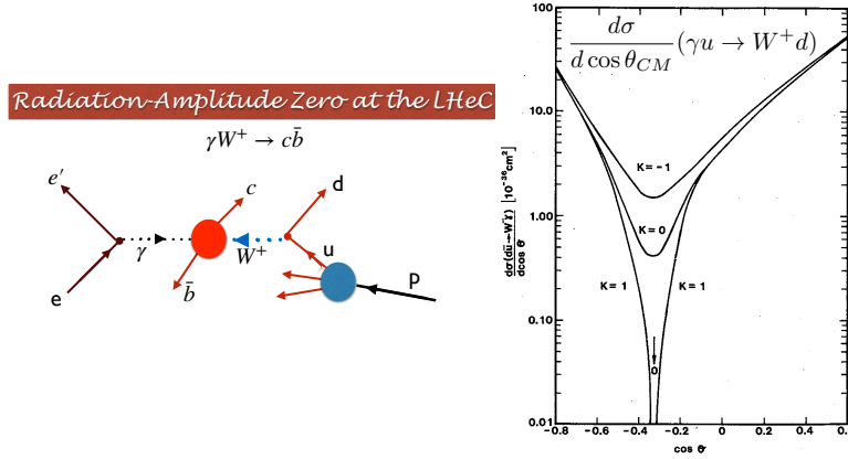
Figure 8.13: The radiation amplitude zero of the Standard Model in \gamma W^+ \rightarrow c \bar{b} and \gamma u \rightarrow W^+ d . The prediction for the angular distribution \frac{d\sigma}{d\cos(\theta_{CM})}(\gamma u \rightarrow W^+ d) is from Ref. [669].
