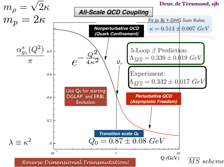
Figure 4.28: Prediction for the running coupling \alpha_{g_1}^s(Q^2) at all scales. At lower Q^2 predictions are obtained from LF Holography and at higher Q^2 from perturbative QCD. The magnitude and derivative of the perturbative and non-perturbative coupling are matched at the scale Q_0 . This matching connects the perturbative scale \Lambda_{\overline{MS}} to the non-perturbative scale \kappa which underlies the hadron mass scale.
