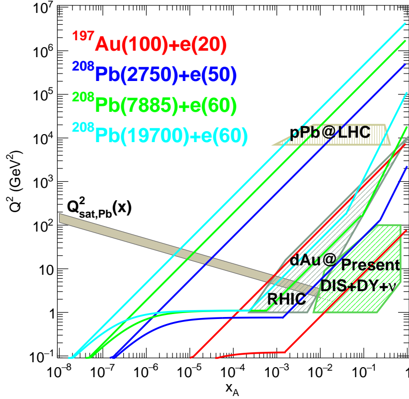
Figure 6.1: Kinematic regions in the x - Q^2 plane explored by different data sets (charged lepton and neutrino DIS, DY, d\text{Au} at RHIC and p\text{Pb} at the LHC) used in present nPDF analyses [495], compared to the ones achievable at the EIC (red), the LHeC (ERL against the HL-LHC beams, dark blue) and two FCC-eh versions (with Pb beams corresponding to proton energies E_p = 20 TeV - green and E_p = 50 TeV - light blue). Acceptance of the detector for the electrons is taken to be 1^\circ < \theta < 179^\circ , and 0.01(0.001) < y < 1 for the EIC (all other colliders). The saturation scale Q_{\text{sat}} shown here for indicative purposes only, see also [496], has been drawn for a Pb nucleus considering an uncertainty \sim 2 and a behaviour with energy following the model in [497]. Note that it only indicates a region where saturation effects are expected to be important but there is no sharp transition between the linear and non-linear regimes.
